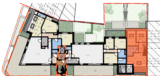
INPLANTINGSPLAN
